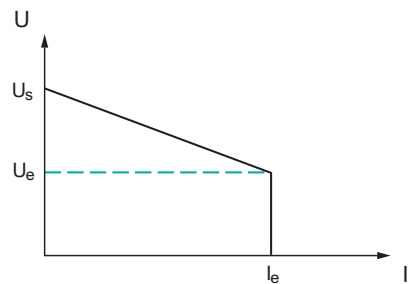
Output characteristic
